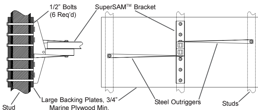
Figure 4: Stud Mounting
