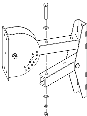
Exploded View
