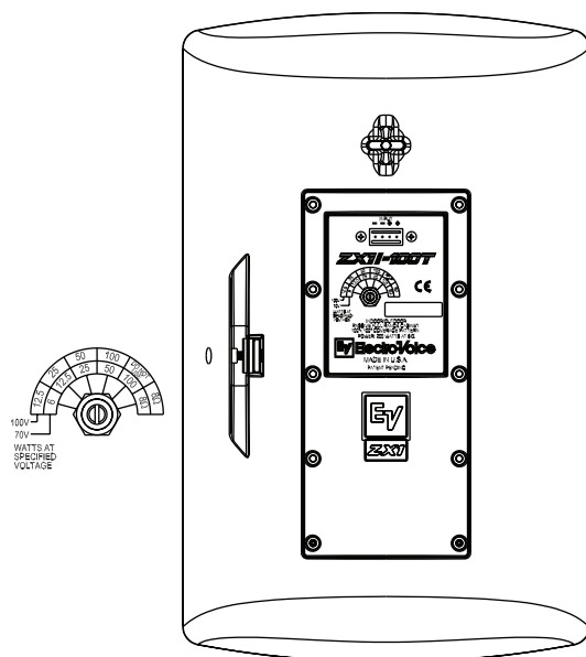
Figure 2.1: Voltage tap selector (ZX1i-90T and ZX1i-100T models only)
