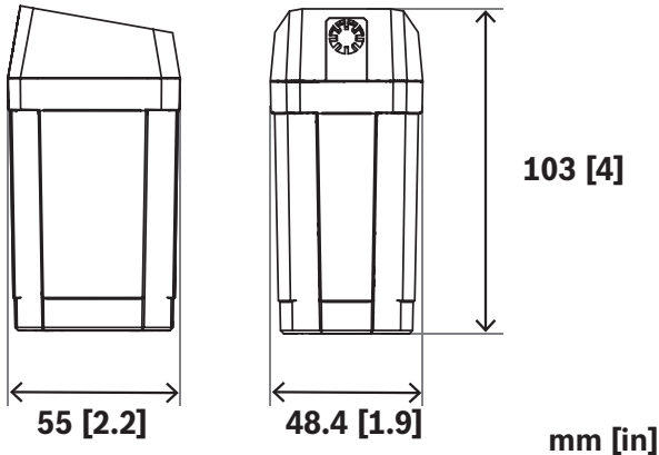
Fig. 3: Subwoofer adapter for EVOLVE-WMK with Phoenix-style connector
