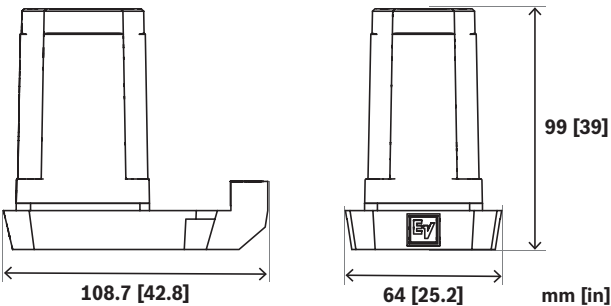
Fig. 2: Column speaker adapter for EVOLVE-WMK with Phoenix-style connector
