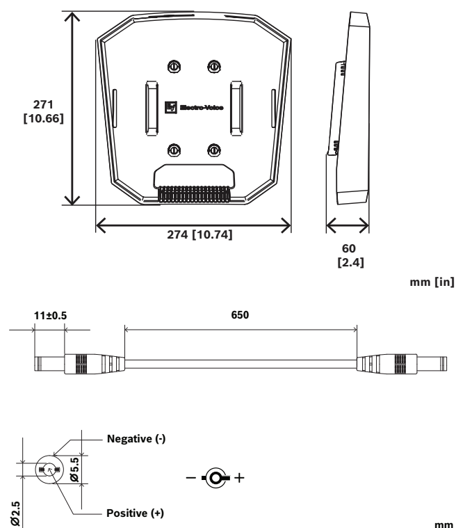
Fig. 1: EVERSE8 DC power cable measurements and polarity
